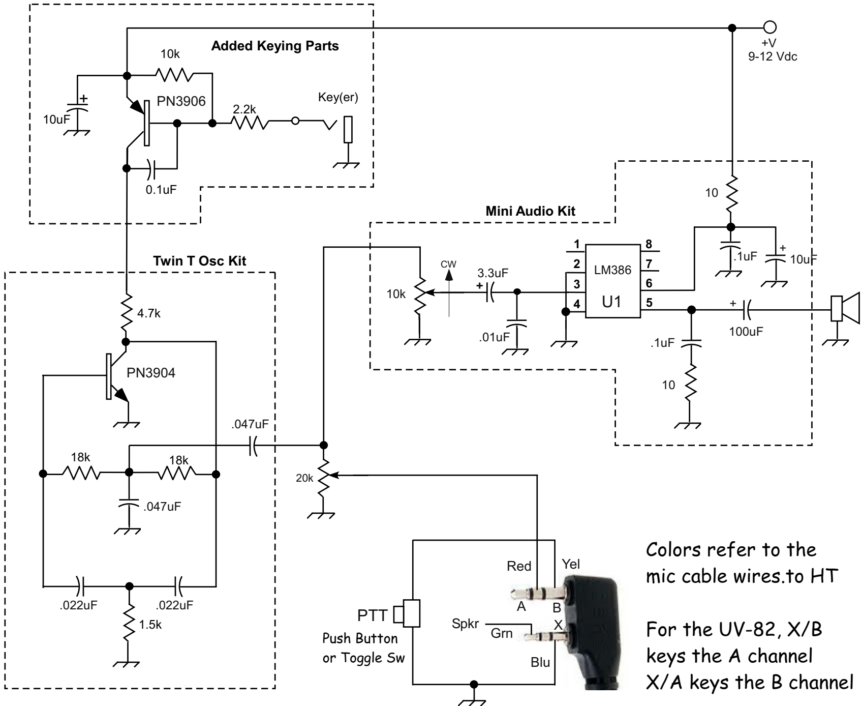
UV-5r/82 MCW Keying Adapter W5USJ dwg 11 Apr 2015
